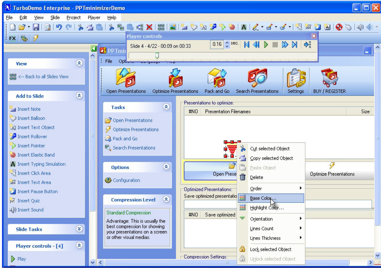
Fig. 1: TurboDemo Screenshot
