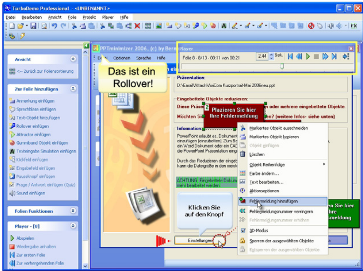
Abb. 1: TurboDemo Screenshot
